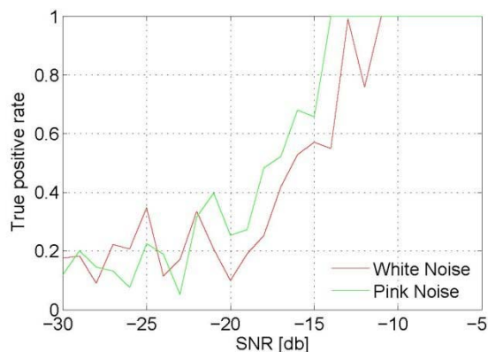
FIGURE 3. Probability of detection versus SNR for Scuba Pro, exploiting a strong feature around 13 kHz
