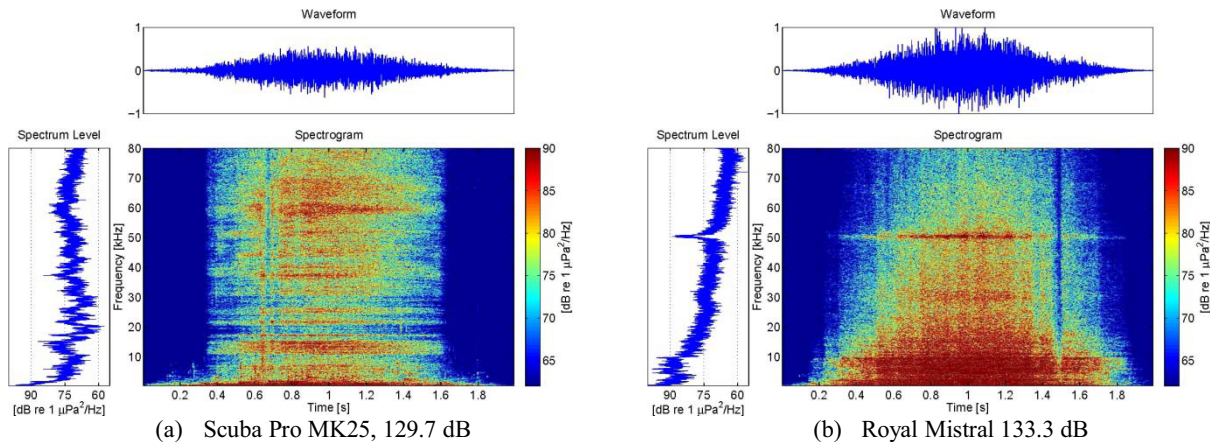
FIGURE 2. Spectrogram (2048 frequency bins), Spectrum Levels and Waveform of tested SCUBA Regulators
